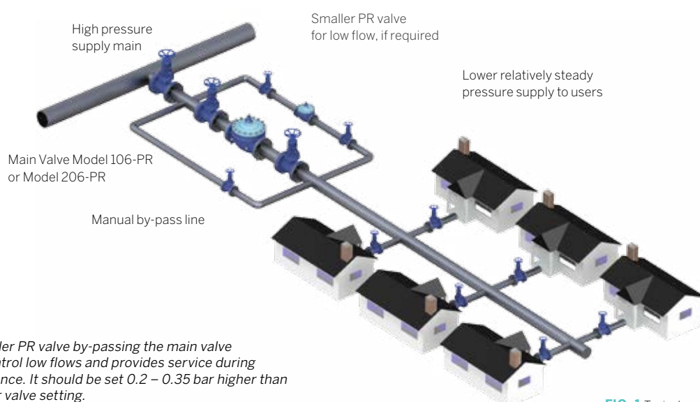
FIG. 1 Typical application
