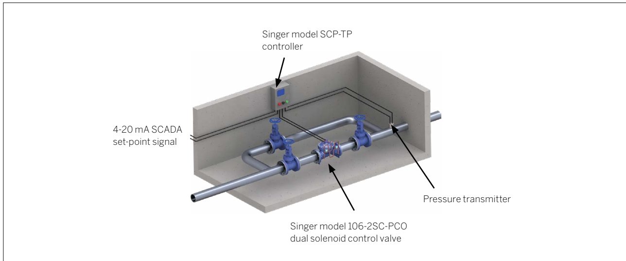
FIG. 1 Typical application
